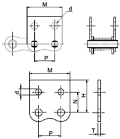
DIN 8187-2 Outer Attachments for European Series
