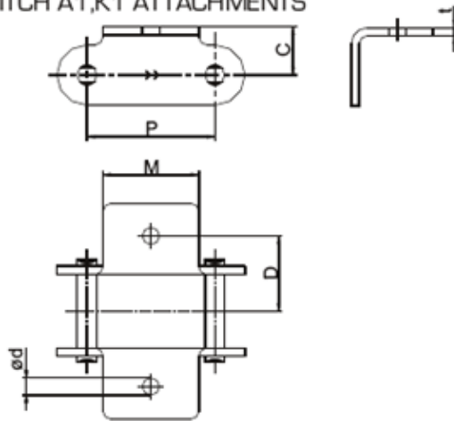
ANSI B 29.4 Outer attachments for American series
