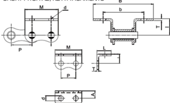
DIN 8187-2 Outer Attachments for European Series
