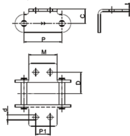
ANSI B 29.4 Outer attachments for American series
